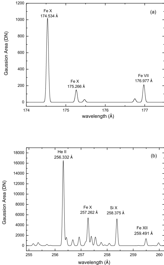
Figure 2. Synthetic Gaussian fitted spectra from the EIS short wave band (a) and long wave band (b) nearby the 257 MIT line (bottom panel) and reference lines (top panel) shown in Fig. 1 for AR2. FWHM= 0.06 Å for short wave band, FWHM= 0.07 Å for long wave band, as recommended in Brown et al. (2008) .
