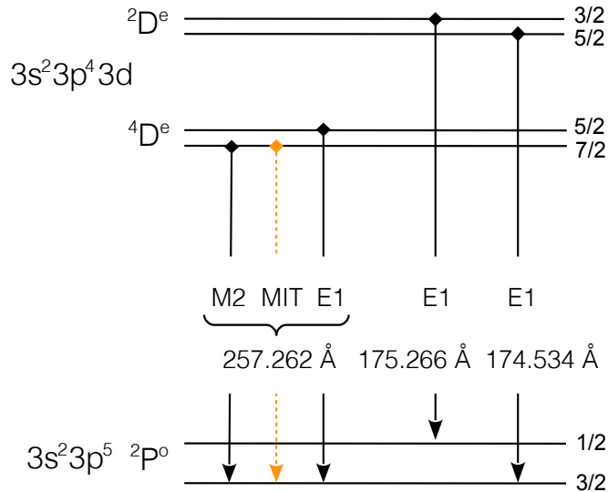
Figure 1. Schematic energy level diagram and decay channels for the levels in \text{Fe}^{9+} that are relevant to the method discussed in this work (see text). Wavelengths are given in Å.
