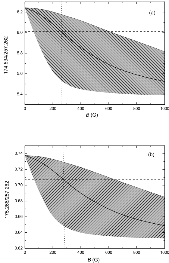
Figure 3. Simulated intensity ratio (black line) of (a) 174.534/257.262 and (b) 175.266/257.262 as a function of the magnetic field in the AR area. The grey shaded area shows the uncertainty caused by the uncertainty in the \Delta E -parameter (see text). The horizontal dashed line is the line ratio measured from HINODE. The vertical dotted line shows our estimated magnetic strength.
